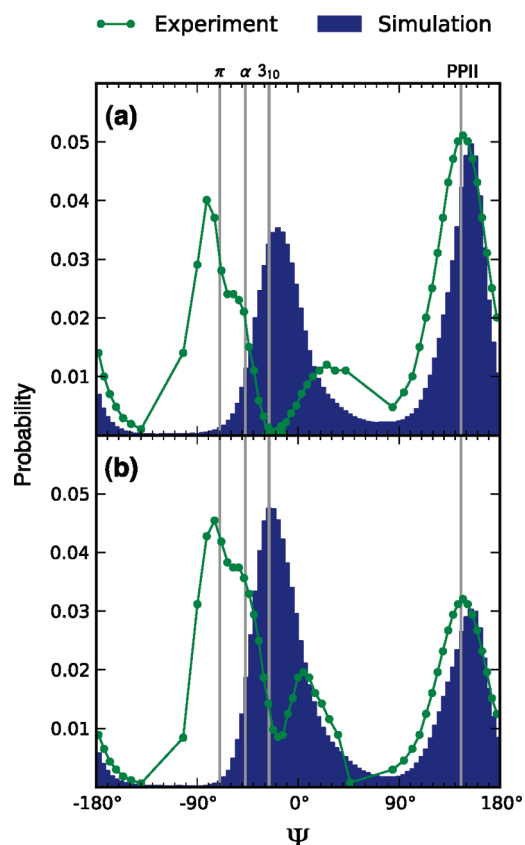
Figure 4. Distributions of backbone \Psi angles for the (a) wild-type and (b) P27S mutant peptides at 30 °C determined from explicit solvent MD simulations (blue) and UVR spectroscopy (green). Source data for these plots are provided in the Supporting Information (Data S1–S4).
